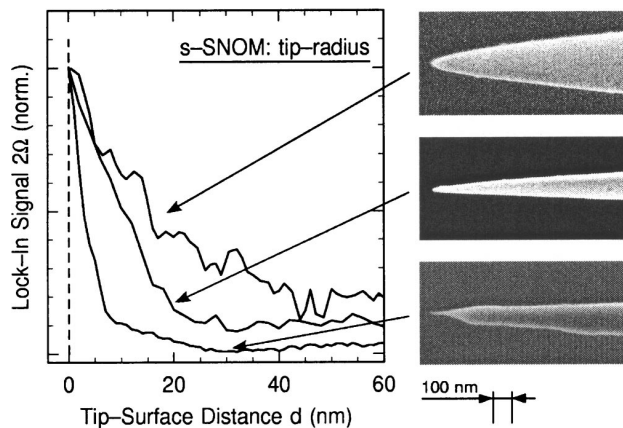
FIG. 2. Normalized tip-sample distance dependence of I_{2\Omega}(d) for tips with different radii of curvature of r \approx 20 nm, r \approx 12 nm, and r \approx 5 nm. The ratio of I_{2\Omega}(0 \text{ nm}) is 1:14:20 with the strongest signal for the r \approx 5 nm tip.
