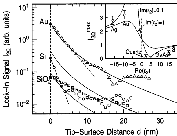
FIG. 3. Variation in optical amplitude I_{2\Omega}(d) for different sample materials showing characteristic distance dependencies representative for metals, semiconductors, or insulators. Inset: I_{2\Omega}^{\text{max}} for d=0 nm vs \text{Re}(\epsilon_2) of the sample material. Solid lines correspond to a simple coupled dipole model.
